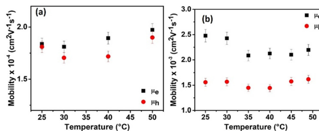
Fig. 7 Temperature dependence of ambipolar charge carrier mobility for compounds (a) 9 and (b) 11 . \mu_{\text{e}} and \mu_{\text{h}} , respectively, represent the electron and hole mobilities.
