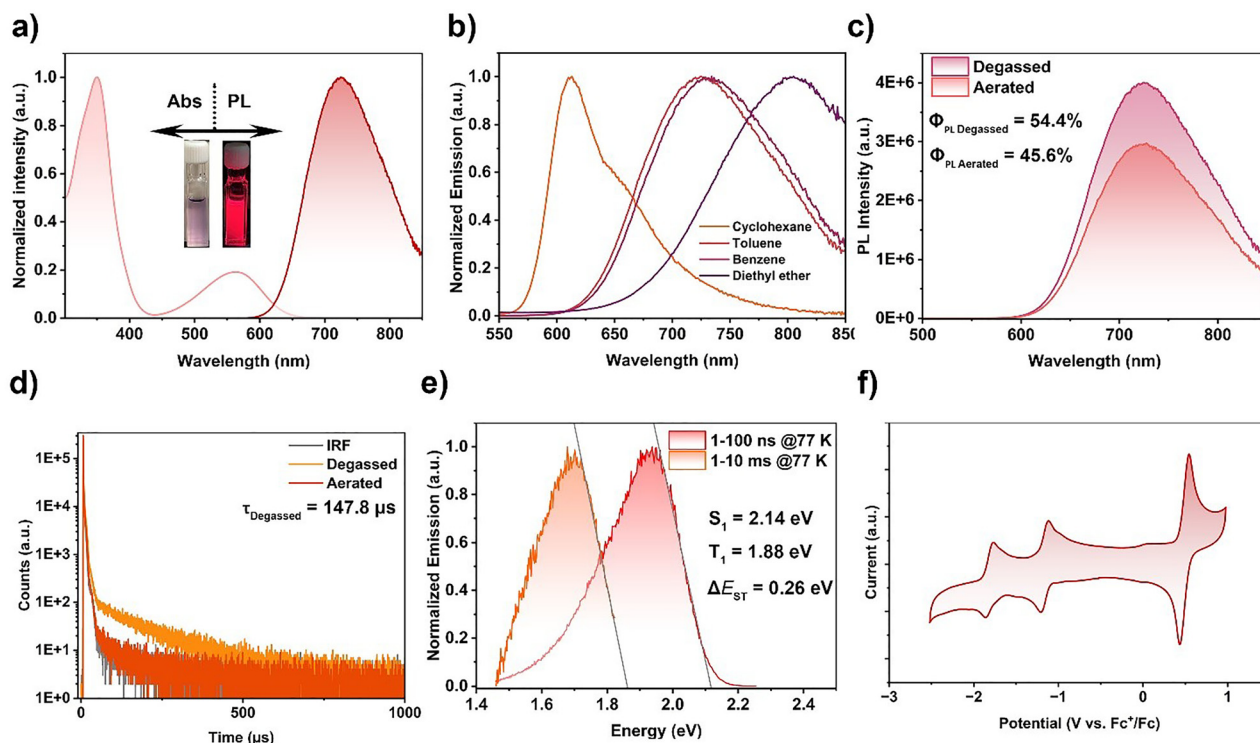
Fig. 1 (a) UV-vis absorption and PL spectra of DPPZ in toluene at room temperature ( \lambda_{exc} = 380 nm, 1.0 \times 10^{-5} M); (b) PL spectra of DPPZ in solvents of varying polarity ( \lambda_{exc} = 380 nm, 1.0 \times 10^{-5} M); (c) PL spectra of DPPZ in degassed and aerated toluene ( \lambda_{exc} = 380 nm, 1.0 \times 10^{-5} M); (d) time-resolved PL decay spectra of DPPZ in degassed and aerated toluene ( \lambda_{exc} = 380 nm, 1.0 \times 10^{-5} M); (e) prompt fluorescence (1–100 ns) and phosphorescence spectra (1–10 ms) recorded in toluene at 77 K of DPPZ ( \lambda_{exc} = 380 nm, 1.0 \times 10^{-5} M); (f) cyclic voltammograms of DPPZ recorded versus Fc^+/Fc at 298 K in o -difluorobenzene under N_2 atmosphere.
