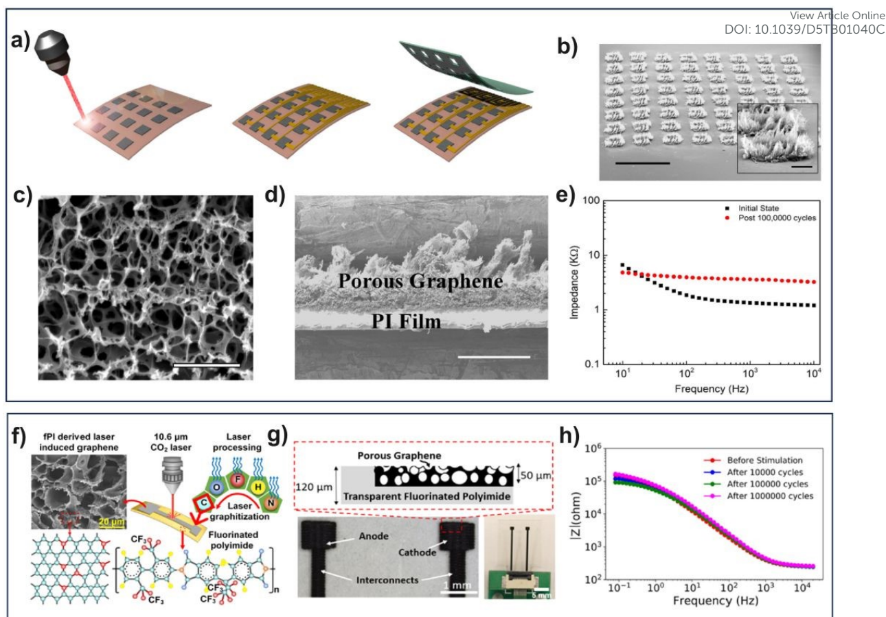
Figure 11 Fabrication process of porous graphene electrode (a). SEM images of the porous graphene array showing the perforated and rough structure of LIG (b-d). The Altered profile of EIS spectrum after 100,000 cycles of biphasic stimulation pulses (e). Reproduced from reference 83 with permission from Nature, Copyright 2016. Preparation of F-doped laser-induced graphene electrodes (fPI-3DPG) from fluorine incorporated polyimide precursor (f,g) and the stable EIS spectrum of fPI-3DPG even after 1 million pulse stimulation cycle (h). Reproduced from reference 76 with permission from American Chemical Society, Copyright 2024.
