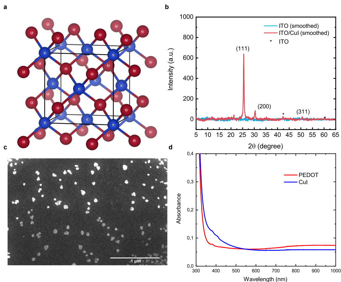
Fig. 1 (a) Schematic representation of the crystal structure of CuI. Cu and I atoms are represented in blue and red, respectively. (b) X-ray diffraction (XRD) pattern of CuI deposited on ITO glass substrates (red) and of the reference ITO glass substrate (blue). (c) SEM image of CuI film. (d) Absorbance spectra of PEDOT: PSS and CuI deposited on ITO.
