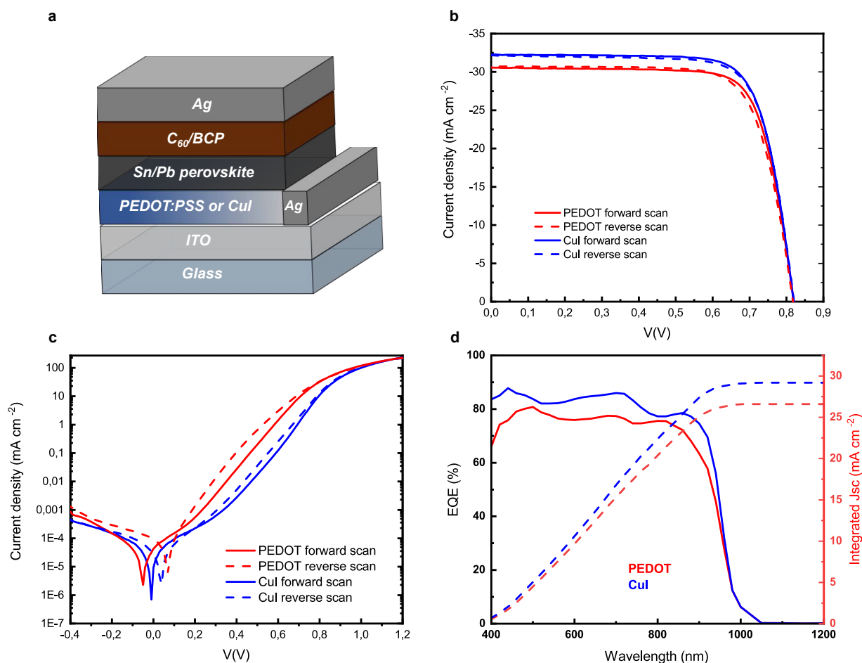
Fig. 3 (a) Device structure of the fabricated p-i-n perovskite solar cell, (b) current density-voltage (J-V) and (c) dark J-V curves of perovskite solar cells fabricated by using PEDOT:PSS (red) and CuI (blue) as HTLs. (d) External quantum efficiency (EQE) as a function of the wavelength and integrated current of the two different structures used.
