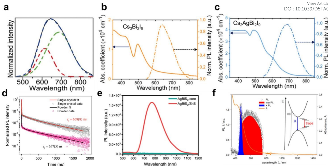
Figure 6. Representative absorption and photoluminescence (PL) characteristics of Ag–Bi PIMs. (a) Deconvoluted PL spectrum showing multiple recombination channels in a representative Ag–Bi PIM, \text{Cs}_2\text{AgBiBr}_6 . Reproduced with the permission from Ref. 127 Copyright 2016, WILEY-VCH. (b) Absorption coefficient and normalized PL intensity of \text{Cs}_3\text{Bi}_2\text{I}_9 , highlighting low absorption near the band edge and broad PL emission. (c) Optical properties of \text{Cs}_2\text{AgBi}_2\text{I}_9 , including absorption onset and broad PL emission indicating sub-bandgap recombination. Panels b and c are reproduced with the permission from Ref. 105 under the terms of the CC-BY license. Copyright 2024, The Author(s), published by Wiley-VCH GmbH. (d) Time-resolved PL decay curves of single crystal and powder samples of \text{Cs}_2\text{AgBiBr}_6 . Reprinted (adapted) with permission from Ref. 125 Copyright 2016, American Chemical Society. (e) PL comparison between \text{AgBiS}_2 core and \text{AgBiS}_2/\text{ZnS} core-shell nanocrystals, revealing strong PL enhancement upon surface passivation with ZnS, indicating suppression of surface trap states. Reproduced from Ref. 47 under the terms of CC-BY 4.0. Copyright 2024, American Chemical Society. (f) Steady-state PL spectrum of \text{AgBiS}_2 NCs (Inset: schematic representing the origin of the trap-assisted PL component of the PL spectrum of the NCs). Reproduced from Ref. 10 under the terms of CC-BY 4.0. Copyright 2023, The authors, published by American Chemical Society.
