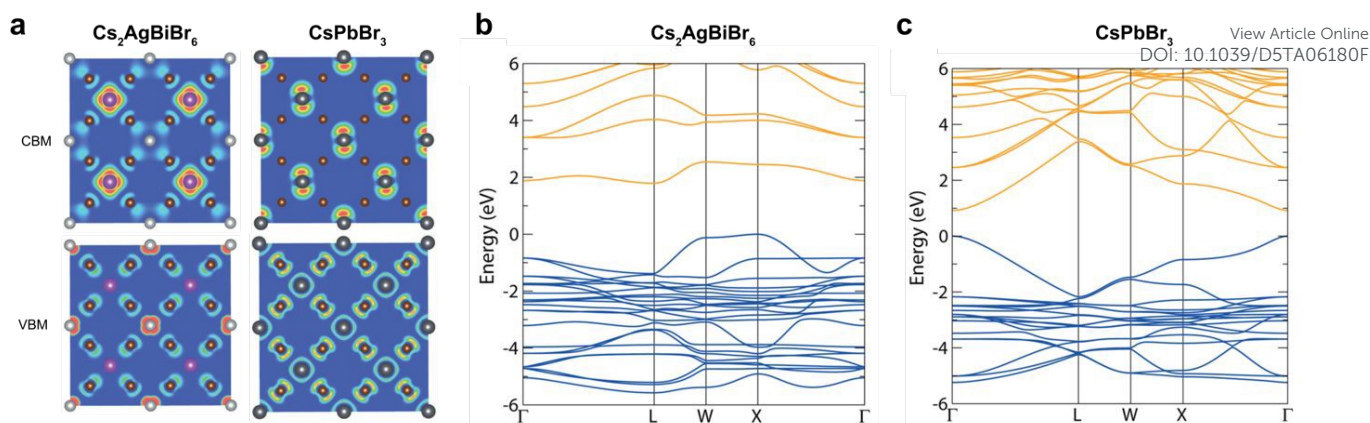
Figure 2. (a) Charge density isosurfaces of the valence band maximum (VBM) and conduction band minimum (CBM), at the Brillouin zone centre. These isosurfaces illustrate the different orbital connectivity in Cs 2 AgBiBr 6 and CsPbBr 3 . While in the former, charge density is localised on Bi atoms in the conduction band and on Ag atoms in the valence band, charge density is more evenly spread in the latter. Ag atoms are in light gray, Bi is in purple, Pb is in dark gray, and Br is in brown. Reproduced with permission from Ref. 57 , licensed under a Creative Commons Attribution (CC-BY) license. (b), (c). HSE06+SOC band structures of Cs 2 AgBiBr 6 and CsPbBr 3 , respectively. Reproduced with permission from Ref. 57 , licensed under a Creative Commons Attribution (CC-BY) license.
