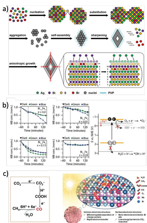
Figure 8. (a) Schematic illustration showing the growth mechanism of AgBiS 2 nanocrystals through anion exchange. Reproduced from Ref. 157 with permission from the Royal Society of Chemistry, Copyright 2024. (b) Methylene Blue photocatalytic degradation by Fe-doped Cs 2 AgBiBr 6 at different doping ratio and process mechanisms. Reproduced from Ref. 158 with permission from Wiley-VCH, copyright 2023. (c) Mechanism of the photocatalytic CO 2 reduction by Rb-doped Cs 2 AgBiBr 6 and effect of the surface atoms substitution. Reproduced from Ref. 159 with permission from Wiley-VCH, copyright 2024.
