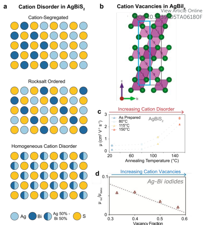
Figure 4. (a) Illustration of different types of cation ordering in \text{AgBiS}_2 . The partial occupancy of the Ag(I), Bi(III) cation sites is represented as fractional filling of the circles at each site. These schematics of \text{AgBiS}_2 structures depict ideal segregated (top), ordered (middle), and homogeneously disordered cases (bottom). Reproduced from Ref. 92 , licensed under a Creative Commons Attribution (CC-BY 4.0) license. (b) Illustration of cation vacancies in \text{AgBi}_4 . Adopting the \text{CdCl}_2 -type structure, \text{AgBi}_4 shows a layered structure with alternating fully occupied and entirely vacant layers. Reproduced from Ref. 87 , licensed under a Creative Commons Attribution (CC-BY) license. (c) Charge-carrier mobility in \text{AgBiS}_2 nanocrystals thin films, as a function of annealing temperature. With increasing temperatures, the increasingly homogeneous CD yields improved charge-carrier mobilities for both delocalised (squares) and localised (triangles) states. Reproduced with permission from Ref. 92 , licensed under a Creative Commons Attribution (CC-BY 4.0) license. (d) Ratio between the mobility of localised and delocalised charge carriers in (\text{AgI})_x(\text{BiI}_3)_{1-x} thin films as a function of the fractional vacancy concentration in the Rudorffite structure. Reproduced from Ref. 60 under the terms of Creative Commons Attribution (CC-BY 4.0) license.
