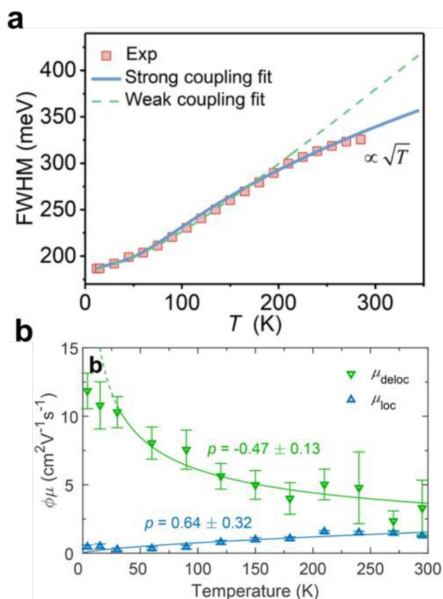
Figure 3. (a) Temperature-dependent photoluminescence (PL) broadening measured for \text{Cs}_2\text{AgBiBr}_6 single crystals. The dashed line indicates the conventional phonon coupling model (weak coupling regime), while the solid line indicates the fit with the Toyozawa strong-coupling model. Reproduced from Ref. 80 , licensed under a Creative Commons Attribution (CC-BY-NC) license. (b) Temperature-dependent mobility for delocalised (green triangles and line) and localised states (blue triangles and line) in \text{Cs}_2\text{AgBiBr}_6 thin films. Reproduced from Ref. 85 under a Creative Commons Attribution (CC-BY 4.0) license.
