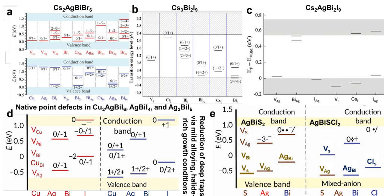
Figure 5. Energy level diagrams and defect energetics in Ag–Bi halides and chalcogenides. (a) Calculated charge transition levels of native point and antisite defects in \text{Cs}_2\text{AgBiBr}_6 , including V_{\text{Cs}} , V_{\text{Ag}} , V_{\text{Bi}} , \text{Bi}_{\text{Cs}} , and \text{Ag}_{\text{Bi}} , with their respective charge states across the bandgap. Reproduced with the permission from Ref. 103 Copyright 2016, WILEY-VCH. (b) Thermodynamic transition levels ( E_{\text{q}}/q' ) of intrinsic point defects in \text{Cs}_3\text{Bi}_2\text{I}_9 , referenced to the valence band maximum (VBM), showing the depth and recombination potential of each defect. Reproduced with the permission from Ref. 104 Copyright 2017, American Chemical Society. (c) Distribution of key defect levels in \text{Cs}_3\text{Bi}_2\text{I}_9 , with mid-gap states such as V_{\text{I}} and \text{Bi}_{\text{Ag}} expected to act as nonradiative recombination centers. reproduced with the permission from Ref. 105 under the terms of the CC-BY license. Copyright 2024, The Author(s), published by Wiley-VCH GmbH. (d) Defect transition levels in \text{Cu}_2\text{AgBiI}_6 (CABI), \text{AgBiI}_4 , and \text{Ag}_2\text{BiI}_5 , where shallow acceptors like V_{\text{Cu}} and V_{\text{Ag}} support p-type conductivity, while deeper defects such as V_{\text{Bi}} , \text{Cu}_{\text{Bi}} , and \text{Ag}_{\text{Bi}} introduce trap states that degrade carrier lifetimes. (e) Comparative defect chemistry in \text{AgBiS}_2 and \text{AgBiS}_2\text{Cl}_2 , where V_{\text{S}} acts as a dominant deep donor in \text{AgBiS}_2 , while V_{\text{Ag}} , V_{\text{Bi}} , and \text{Ag}_{\text{Bi}} serve as acceptor-type defects. In \text{AgBiS}_2\text{Cl}_2 , halide incorporation introduces additional defects such as V_{\text{Cl}} and mixed-anion substitutions ( \text{S}_{\text{Cl}} , \text{Cl}_{\text{S}} ), modifying the defect landscape and potentially mitigating deep-level recombination pathways. Panels d and e were fabricated primarily based on the reported defect energy level data presented in the Ref. 70,106,107 and Ref. 92,107–109 , respectively.
