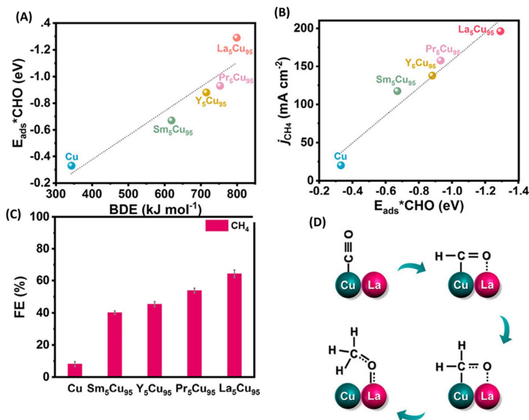
Fig. 5 (A) Relationship between calculated *CHO adsorption energy (energy required to convert one molecule from the lowest adsorbed state to the lowest gaseous state) and the bond dissociation enthalpy (BDE) of the metal–oxygen bond. (B) Relationship between the partial current density of CH 4 at a total current density of 300 mA cm -2 (in CO 2 -saturated 1 M KOH solution) and the adsorption energy of *CHO for Cu and M 5 Cu 95 electrocatalysts. (C) FE of CH 4 on Cu and M 5 Cu 95 electrocatalysts at a total current of 300 mA cm -2 . (D) Proposed reaction pathways of the ECO 2 RR to CH 4 on the La 0.5 Cu 0.5 surface. Reproduced from ref. 102 with permission from the American Chemical Society, copyright 2023.
