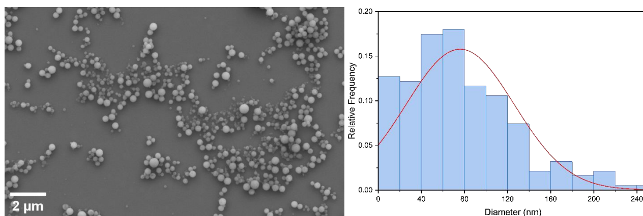
Figure 2. SEM image of the sample Zr 4 -20 (on the left) and average size-distribution (on the right).
