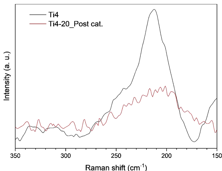
Figure 4. Comparison of the Raman spectra of Ti 4 oxocluster (black line) and Ti 4 -20 recovered after the catalysis (red line).
