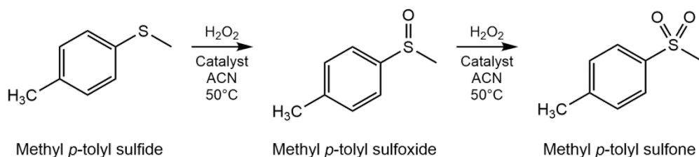
Figure 3. Scheme of the oxidation reaction of methyl p -tolyl sulfide ( S ) to the corresponding sulfoxide ( SO ) and sulfone ( SO 2 ).
