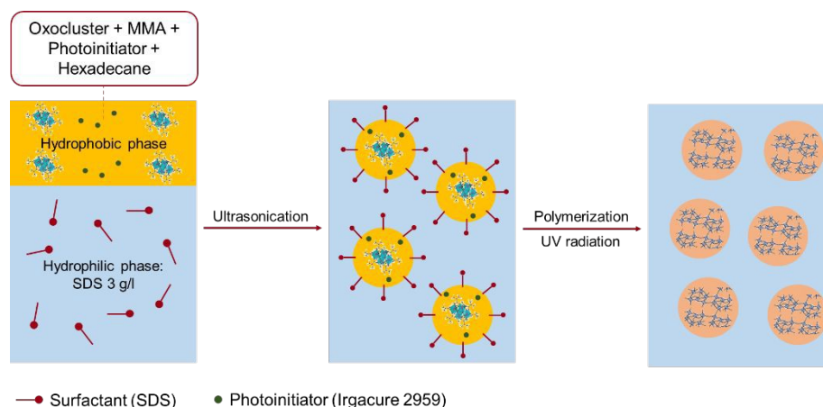
Figure 1. Schematic representation of the miniemulsion polymerization process carried out to obtain oxocluster-based hybrid nanoparticles.
