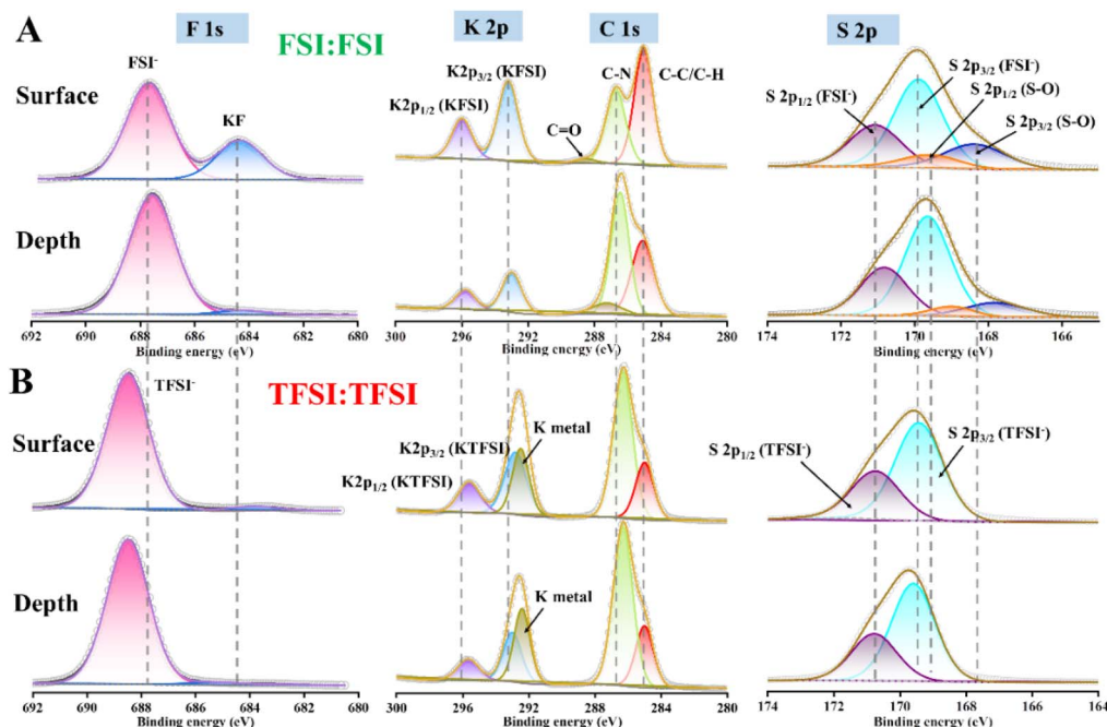
Fig. 6 XPS of the K metal surface and bulk (depth of 8 nm, Ar + etching speed of 0.8 nm min -1 ) after immersing for 28 days in (A) KFSI:Pyrr 12 O 1 FSI or (B) KTFSI:Pyrr 12 O 1 TFSI solutions (the grey open points represent the experimental data, and the solid lines represent the fitting results).
