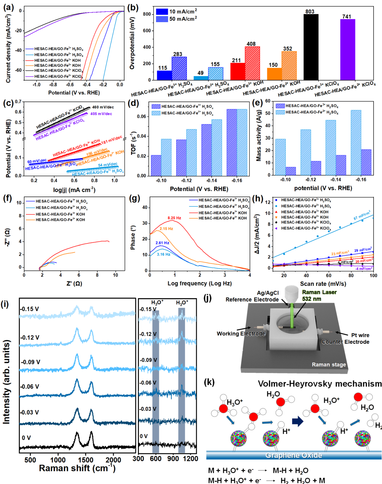
Fig. 4 (a) HER polarization graphs of HESAC-HEA/GO-Fe 2+ and HESAC-HEA/GO-Fe 3+ in 0.5 M H 2 SO 4 , 1.0 M KOH, and 0.1 M KClO 4 solutions at 5 mV s -1 , (b) η at 10 and 50 mA cm -2 , (c) Tafel slope, (d) TOF, (e) mass activity, (f and g) Nyquist and Bode plots, (h) C dl plot, (i) in situ Raman spectra of the HESAC-HEA/GO-Fe 2+ electrocatalyst in 0.5 M H 2 SO 4 during HER process under different potentials, (j) schematic of the in situ electrochemical Raman setup, and (k) proposed HER pathway over the HESAC-HEA/GO-Fe 2+ electrocatalyst.
