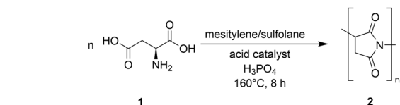
Scheme 1 Thermal polycondensation of aspartic acid 1 to polysuccinimide (PSI) 2.
