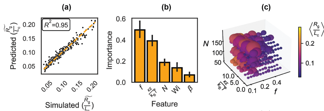
Fig. 6 Analysis of importance of input parameters based on polynomial regression. (a) Predicted versus actual \left(\frac{\widetilde{R}_g}{L_c}\right) . Each data point corresponds to the set of chains that share the same standard parameter space values. (b) Parameter importance by feature permutation. The data provides the median R^2 change from 1000 random shuffles per variable, with error bars indicating the interquartile range. A larger value indicates greater importance. (c) Three-dimensional scatter of the top three predictors f , \frac{\kappa E}{k_B T} , and N , in which the color of each sphere denotes \left(\frac{\widetilde{R}_g}{L_c}\right) and its radius corresponds to the interquartile range. \left(\frac{\widetilde{R}_g}{L_c}\right) is computed for each point in the standard parameter space, and spheres are spaced slightly to separate each (\beta, Wi) combination associated with the same \left(f, \frac{\kappa E}{k_B T}, N\right) .
