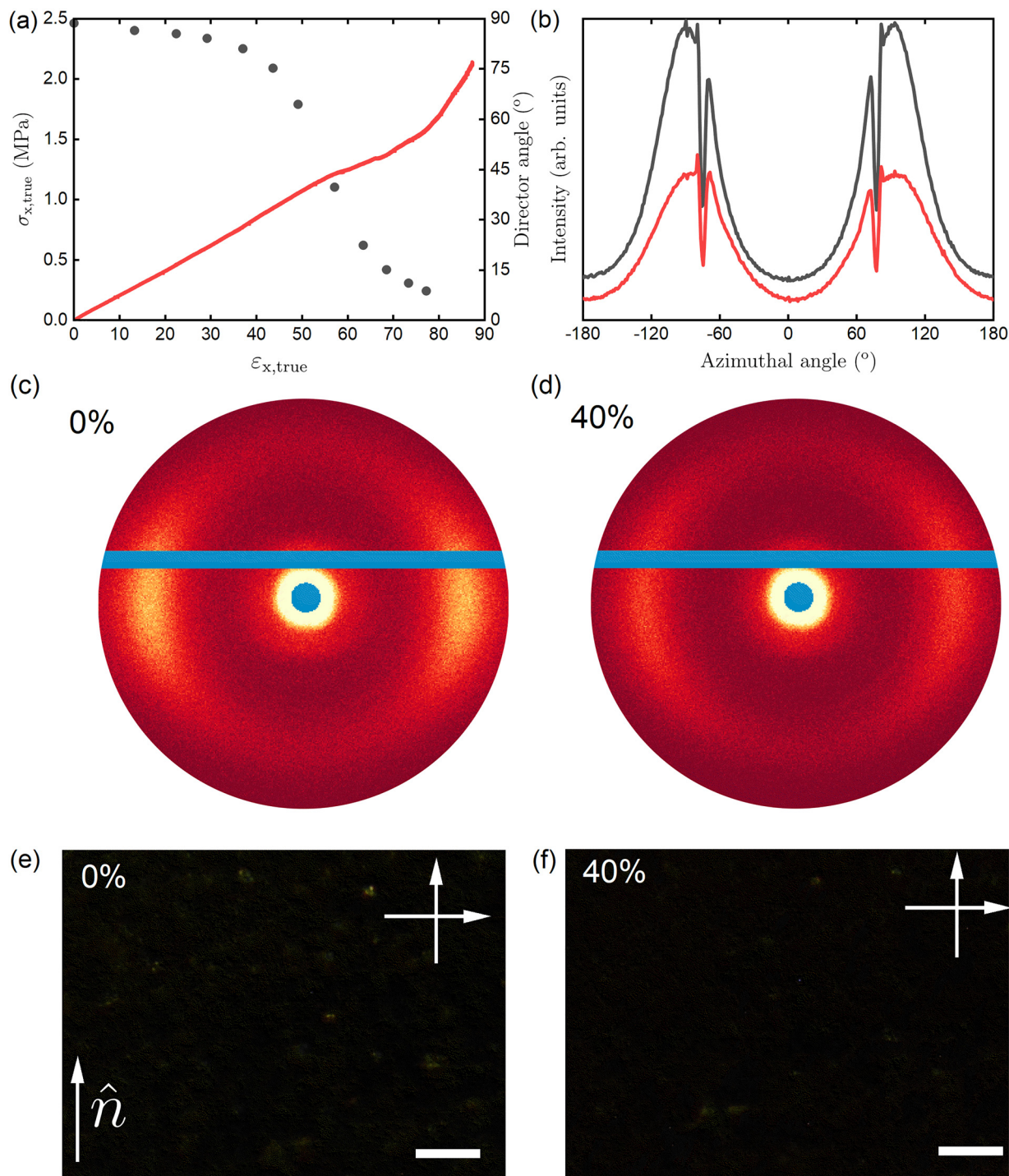
Fig. 7 (a) Stress–strain response of the 1× LCE at a strain rate of 0.1\% \text{ min}^{-1} plotted as a function of true-stress ( \sigma_{x,true} ) and true-strain ( \epsilon_{x,true} ) (red line) and in-plane projection of the director angle as a function of strain as determined via simultaneous observations with crossed polarizers (black circles). (b) X-ray scattering profile as a function of azimuthal angle for the 1× sample under \epsilon_{x,true} = 0\% (black) and \epsilon_{x,true} = 40\% (strain). (c) and (d) 2D X-ray scattering image of the 1× sample at \epsilon_{x,true} = 0\% and \epsilon_{x,true} = 40\% , respectively. (e) and (f) Polarised optical microscopy images of the 1× sample at \epsilon_{x,true} = 0\% and \epsilon_{x,true} = 40\% , respectively. The arrows in (e) and (f) show the direction of the polariser and analyser, \hat{n} defines the orientation of the director in the unstrained sample. Scale bar = 75 \mu\text{m} .
