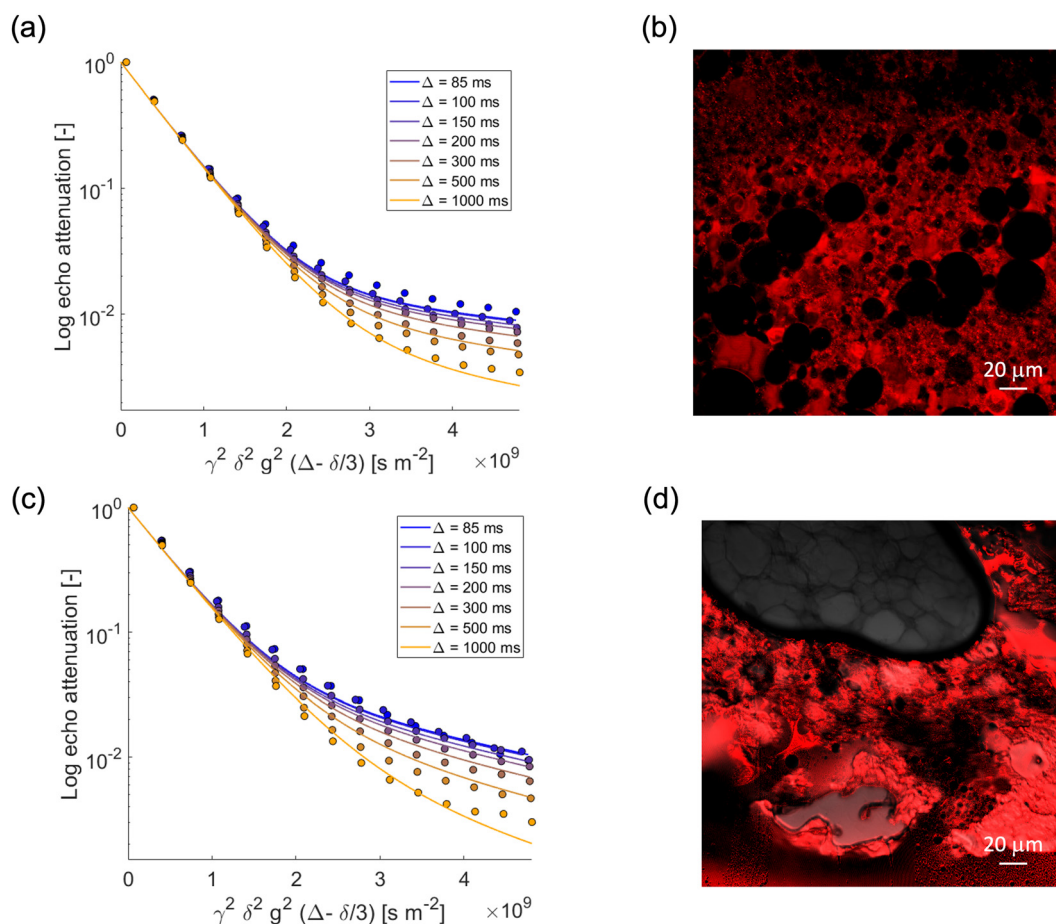
Fig. 3 PGSTE log attenuation plots for (a) water in S/G 1% , (c) water in S/G 2% , at different observation times \Delta = [85, 100, 150, 200, 300, 500, 1000] ms. Solid lines are fittings obtained using eqn (2). (b) and (d) Confocal images of S/G 1% and S/G 2% , respectively. Rhodamine B has been used as fluorescent dye.
