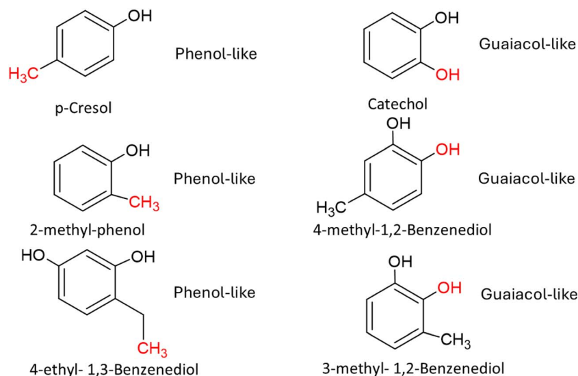
Fig. 5 Some of the main compounds in \text{WS}_{\text{aq}} and \text{PW}_{\text{aq}} and their classification in the system. The functional groups highlighted in red indicate the classification reasoning.
