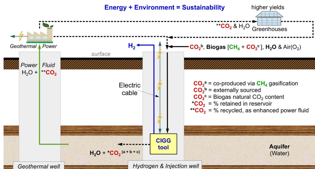
Fig. 8 An Illustration of a wellbore utilizing a wellbore reformation tool within a CIGG Completion. CO 2 a = CO 2 generated by reformation of methane, CO 2 b = CO 2 obtained from external industry sources, CO 2 c = the natural CO 2 content held within biogas, *CO 2 = the % of the injected CO 2 that is retained within the reservoir, **CO 2 = the % of the injected CO 2 that is recirculated within the power fluid.
