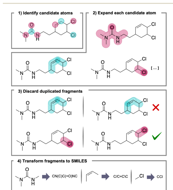
Fig. 2 Scheme and example of the application of the fragmentation algorithm used in the present work.
