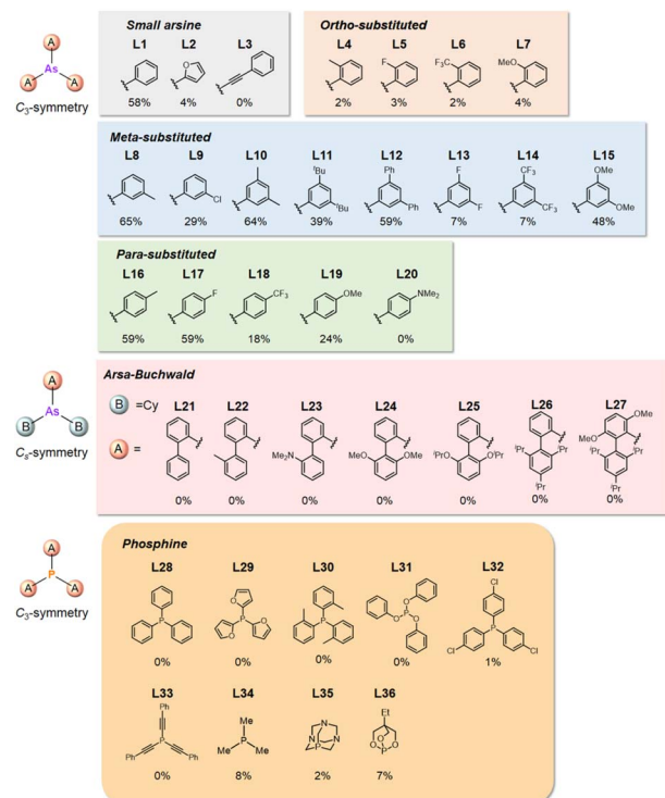
Fig. 2 o -, m -, and p -substituted C_{3v} and C_{2v} -type arsine and phosphine ligands. The NMR yield of the difunctionalized product 1 (Scheme 1) is shown below each structure.
