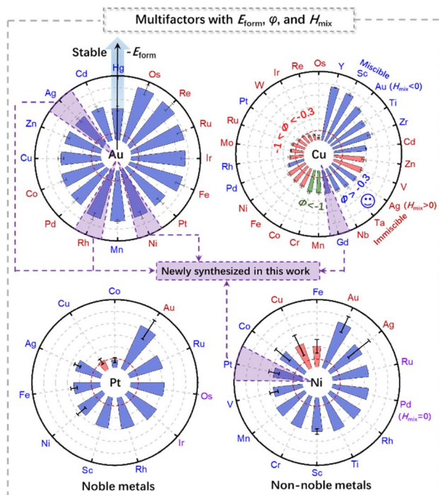
Fig. 8 The accessibility prediction via E_{\text{form}}^{\text{ML}} , \phi , and H_{\text{mix}} for the bimetallic pairs comprising noble metals (Au/M and Pt/M) and base metals (Cu/M and Ni/M) predicted by machine learning.
