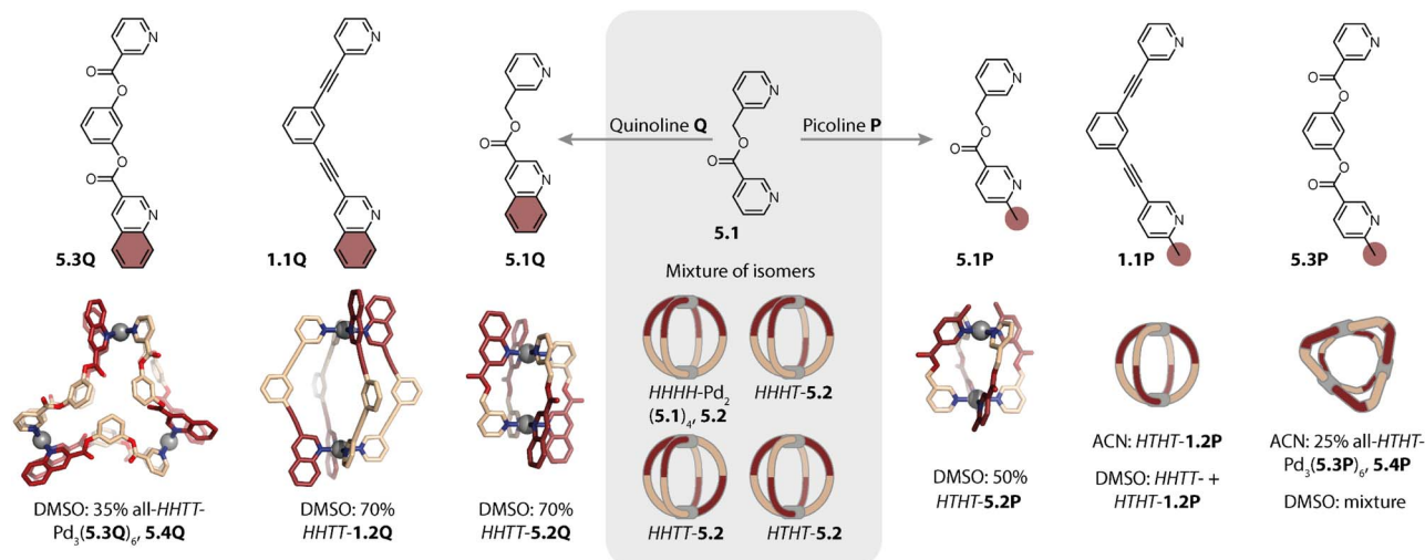
Fig. 20 Biasing the self-assembly of asymmetric ligands by introducing steric constraints on the donor site. (Left) For quinoline-equipped ligands the HHHT-isomer is favoured in DMSO. (Middle) Bis-pyridyl ligand 5.1 assembles to form a mixture of different isomers. (Right) For picolyl-equipped ligands, there is a bias towards HTHT-isomers.
