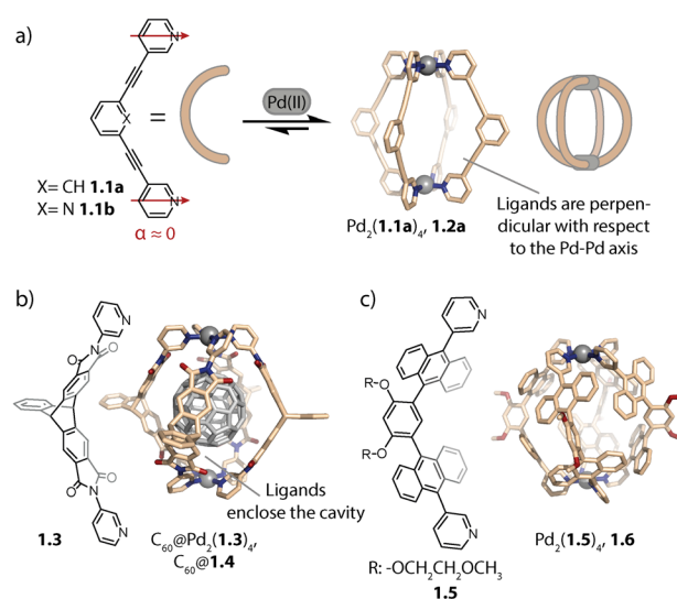
Fig. 1 (a) Self-assembly of lantern-shaped cage 1.2a . (b) Capsule 1.4 based on a triptycene-derived ligand, encapsulating a \text{C}_{60} fullerene. (c) Capsule 1.6 based on ligands with anthracene panels.
