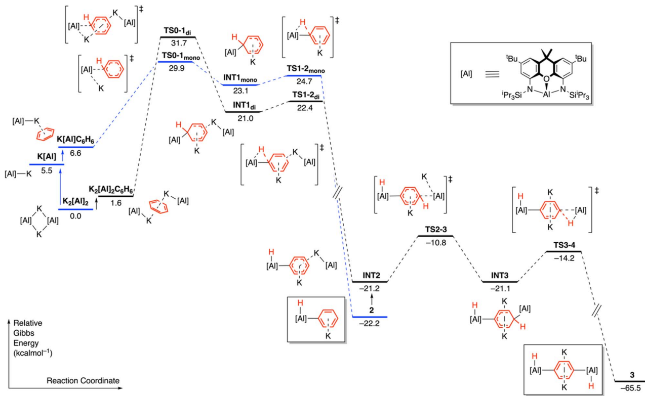
Fig. 3 Gibbs free energy profile (PBE0-D3 BJ -CPCM(benzene)/Def2-TZVPP//PBE0-D3 BJ /BS1) for the reaction between the transiently generated K_n[Al(TIPS)NON] , ( n = 1, 2 ) alumanyl complex and benzene to give C–H activation complexes 2 and 3. Relative Gibbs free energies are presented in kcal mol −1 . Monomeric pathway highlighted in blue.
