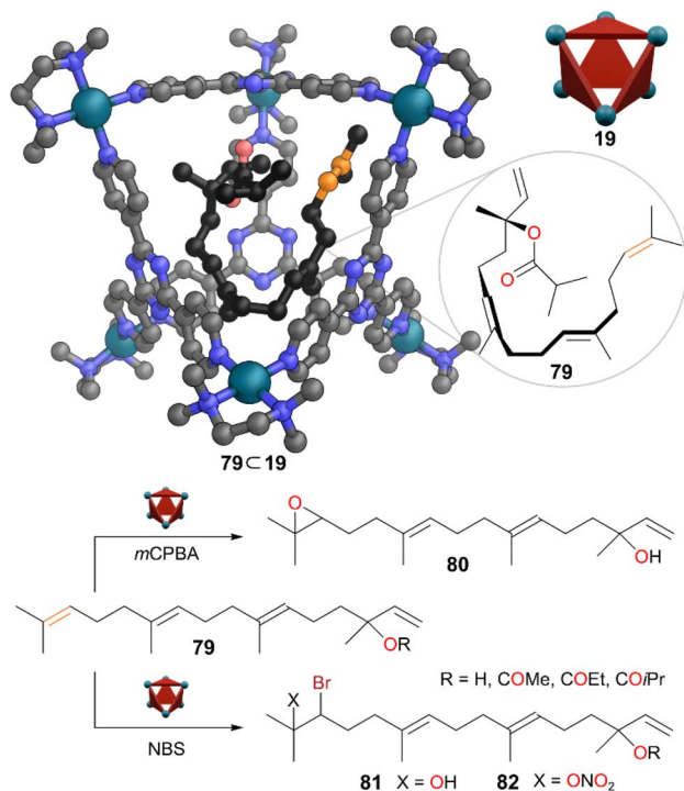
Fig. 22 Representation of the SCXRD structure of cage 79 \subset 19 , and selective reactions of terpene 79 to products 80–82 . Disorder, solvent, hydrogen atoms, and counter anions have been omitted for clarity. Colour: C = grey or black, N = blue, O = red, Pd = turquoise, Br = brown, reactive alkene carbons = orange.
