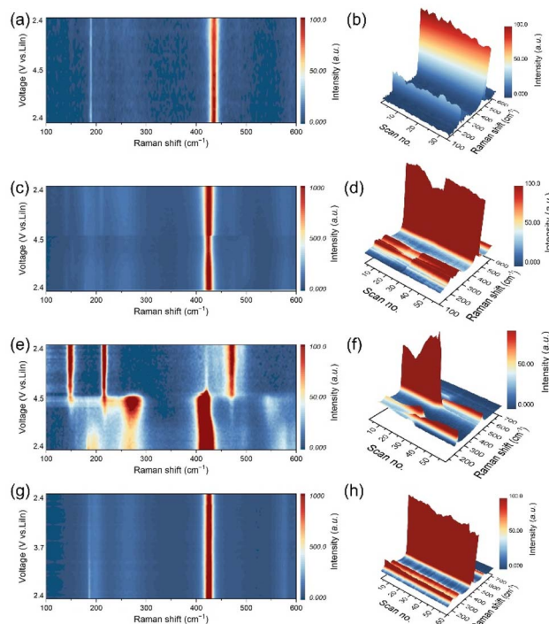
Fig. 2 The in situ Raman spectra of (a and b) LPSCl-VGCF|LPSCl|LiIn, (c and d) uncoated LNMO-LPSCl-VGCF|LPSCl|LiIn, (e and f) LTA@LNMO-LPSCl-VGCF|LPSCl|LiIn, and (g and h) LCO-LPSCl-VGCF|LPSCl|LiIn cells from two-dimensional and three-dimensional views, respectively. The positions for Raman signal collection are the LPSCl-rich area far from the cathode active particle/LPSCl particle interface in the composite cathode.
