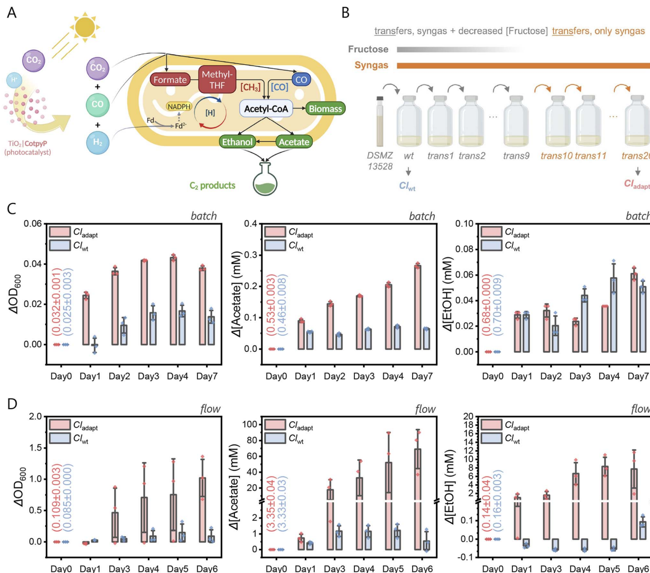
Fig. 1 Adaptive laboratory evolution (ALE) of C. ljungdahlii . (A) Schematic illustration of the syngas-fermenting metabolic pathways in C. ljungdahlii ( Cl ), including integration with photocatalytic syngas production. [\text{CH}_3] (red color), methyl branch; [\text{CO}] (blue color), carbonyl branch. (B) Schematic summary of the ALE process. The wild-type strain ( Cl_{wt} ) was adapted to a syngas environment through gradual fructose reduction and removal over 20 transfers, resulting in the adapted strain ( Cl_{adapt} ). (C) Comparative analysis of growth and \text{C}_2 product generation (acetate and ethanol) between Cl_{adapt} and Cl_{wt} under batch gas purging conditions (syngas purging for 30 min daily, 112 mL headspace). (D) Similar comparative analysis under continuous gas flow conditions (10 mL syngas per min). Growth conditions: ATCC Medium 1754 (pH 5.9), 37 °C with 150 rpm mixing. Numbers in brackets indicate the values at the start of the experiment.
