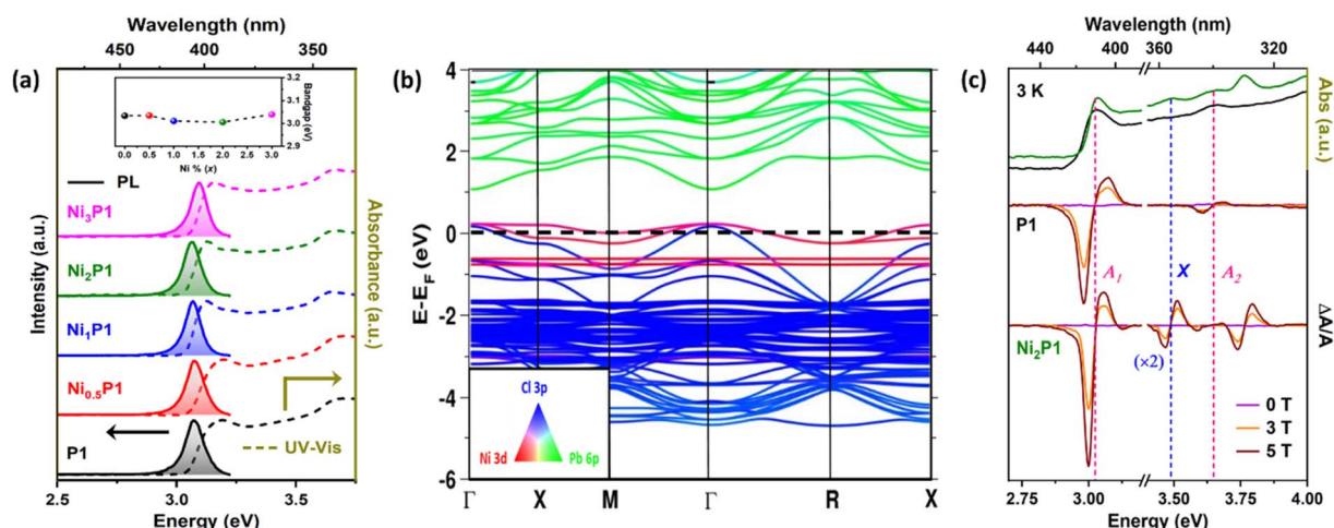
Fig. 2 Optical and electronic properties: (a) room temperature absorption and emission spectra of undoped (P1) and various Ni-doped CsPbCl 3 (Ni x P1; x = 0, 0.5, 1, 2, 3) NCs with the inset of bandgap variation with different Ni-percentage (dashed line guides to the eye) showing a bowing effect. (b) Orbital projected band structure of Ni-doped CsPbCl 3 with considering spin-orbit coupling (SOC). Red, green, and blue colors represent Ni 3d, Pb 6p, and Cl 3p atomic orbitals respectively, while intermediate colors indicate the extent of mixing or hybridization of these orbital contributions. Band structure confirms significant hybridization of Ni 3d and Cl 3p orbitals near the VBM at T point. (c) MCD spectra of P1 and Ni 2 P1 with their absorption at temperature 3 K with varying magnetic field (0, 3, and 5 T). The presence of extra differential peak (X) confirms the Ni 2+ -induced exchange interaction.
