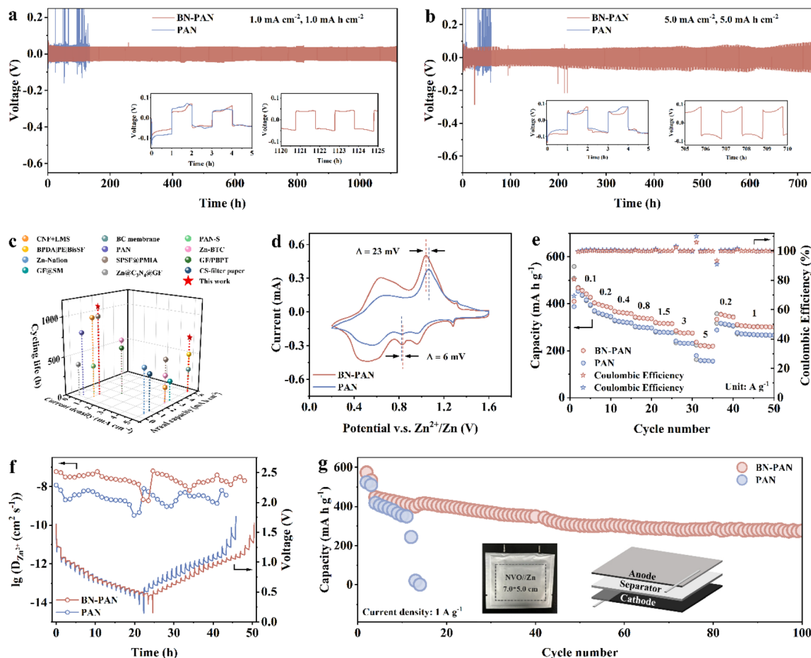
Fig. 4 Electrochemical performance of BN-PAN and PAN separators. The cycling performance of Zn//Zn cells at (a) 1.0 mA cm -2 with 1.0 mA h cm -2 and (b) 5.0 mA cm -2 with 5.0 mA h cm -2 using the BN-PAN separator and PAN separator. (c) The comparison among our BN-PAN separator and previous reports. (d) The CV curves at a scan rate of 0.2 mV s -1 , (e) the rate performance at a current density from 0.1 A g -1 to 5.0 A g -1 , (f) the charge-discharge GITT curves at a current density of 0.1 A g -1 and the corresponding Zn 2+ coefficients of Zn//NVO full cells, and (g) the cycling stability of pouch cells at a current density of 1.0 A g -1 .
