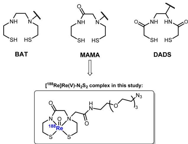
Fig. 1 Examples of \text{N}_2\text{S}_2 chelators for chelating ^{99\text{m}}\text{Tc}(\text{v}) and ^{186/188}\text{Re}(\text{v}) , and the [^{188}\text{Re}]\text{Re}(\text{v})-\text{N}_2\text{S}_2 complex used in this study.
