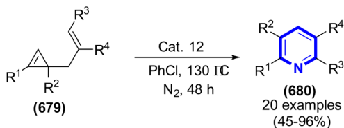
Scheme 189 Synthesis of pyridines catalyzed by Cat. 12.
