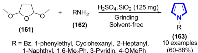
Scheme 44 Synthesis of N -substituted pyrroles catalyzed by H 2 SO 4 SiO 2 (SSA).
