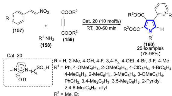
Scheme 43 Synthesis of tetrasubstituted pyrroles catalyzed by Cat. 20.
