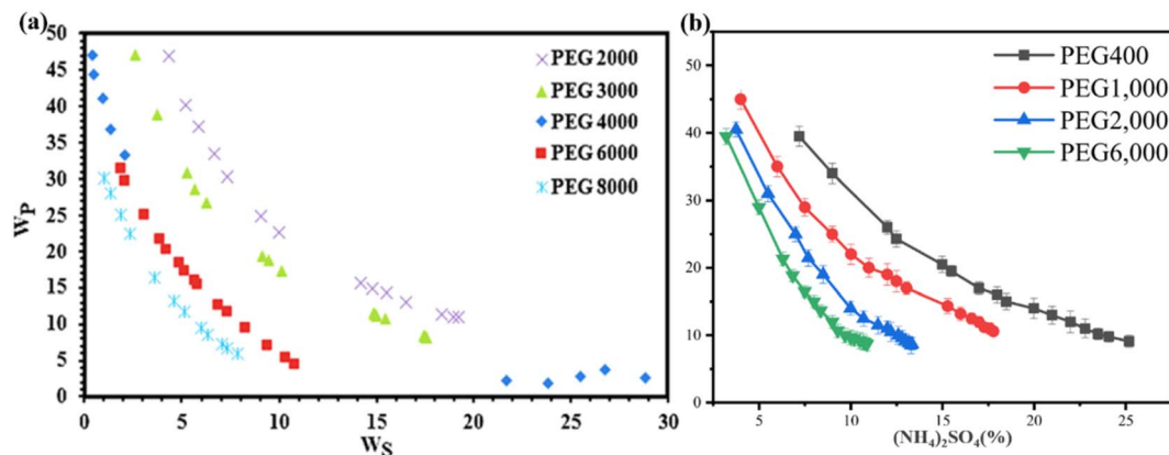
Fig. 3 (a) Experimental binodal data for the phase diagram of PEG + \text{ZnSO}_4 + water system at pH = 4.70, T = 298.15 K, and various molecular masses of PEG (2000, 3000, 4000, 6000, 8000). 39 (b) Phase diagrams of PEG with different molecular weights and (\text{NH}_4)_2\text{SO}_4 in the ATPS in the presence of \text{Tl(I)} and \text{U(VI)} (both were 10 \text{ mg L}^{-1} ). 40
