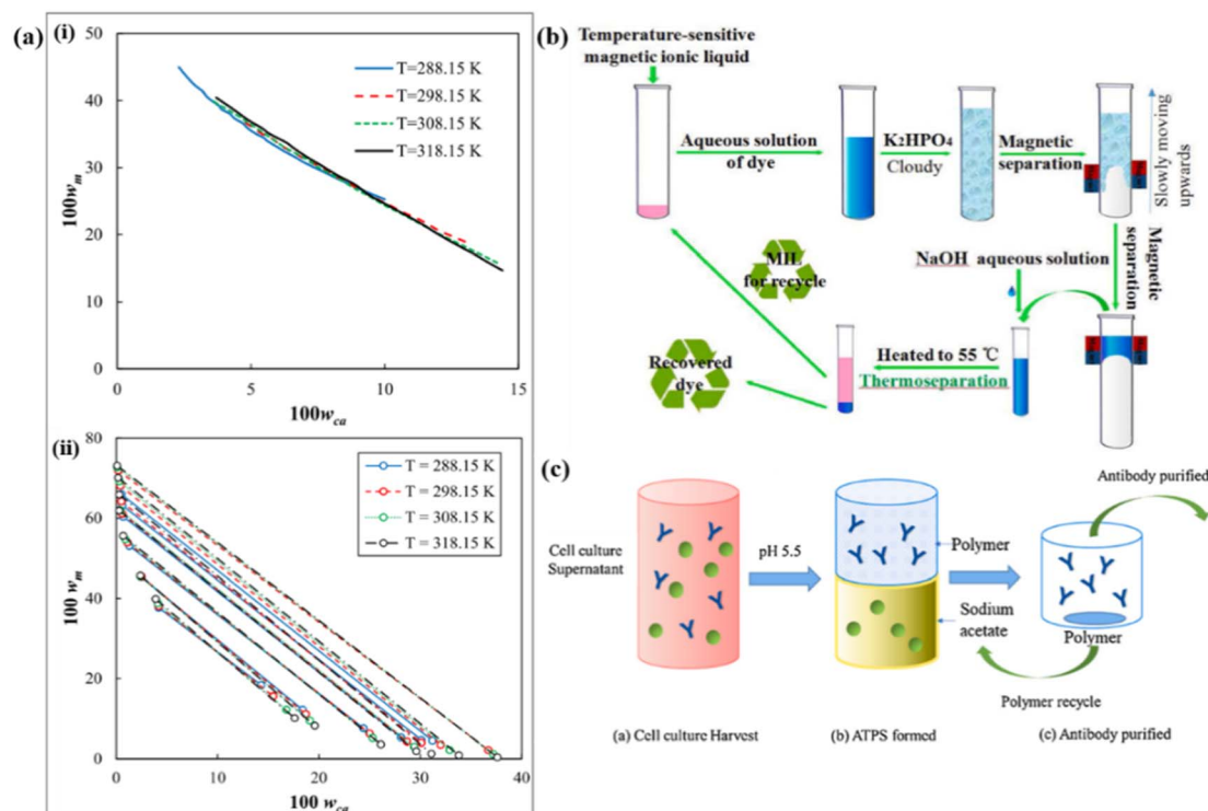
Fig. 5 Comparison of the (a-i) binodal curves and (a-ii) tie-lines for isopropanol + trisodium citrate + water ternary systems at T = 288.15, 298.15, 308.15, \text{ and } 318.15 \text{ K} . 43 (b) Schematic removal and recovery process of triphenylmethane dye. 44 (c) Process of antibody IgG201 partition by pH-ATPS. 45
