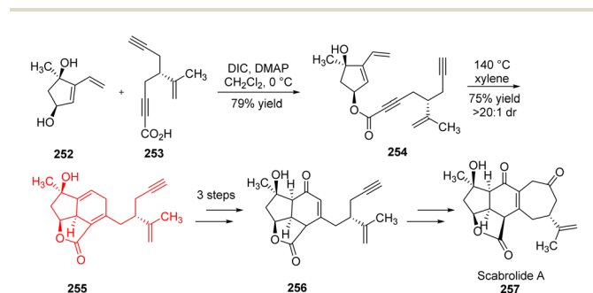
Scheme 32 Total synthesis of scabrolide A ( 257 ). 78
