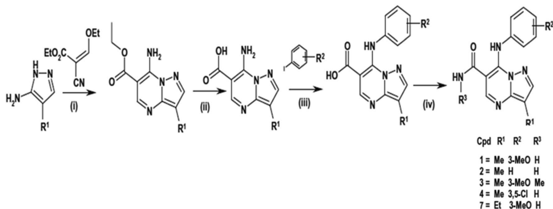
Scheme 22 (i) 3-Amino-4-alkyl pyrazole, ethyl (ethoxymethylene)cyanoacetate (1 equiv.), AcOH, reflux, 4 h, yield: 60%; (ii) NaOH (10 equiv.), EtOH, reflux, 4 h, yield: 62%; (iii) ArI (3 equiv.), CuI (1 equiv.), proline (1 equiv.), K 2 CO 3 (3 equiv.), DMF, microwave, 110 °C, 2 h, yield: 5–35%; (iv) 1-hydroxybenzotriazole (HOBt, 3 equiv.), 1-ethyl-3-(3-dimethylaminopropyl)carbodiimide (EDCI, 3 equiv.), R 3 NH 2 (excess), DMF, room temperature, 2 h, yield: 8–33%. 110
