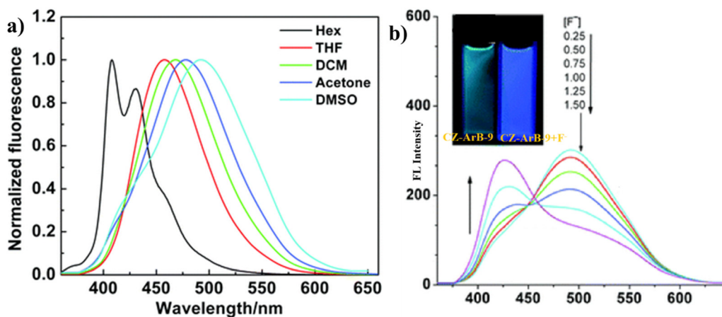
Fig. 6 (a) Fluorescence spectra of CZ-ArB-9 with varying polarity of solvents. (b) Fluorescence titration spectra of CZ-ArB-9 in DMSO upon gradual addition of \text{F}^- . Reproduced with permission from ref. 105. Copyright 2012 Royal Society of Chemistry.
