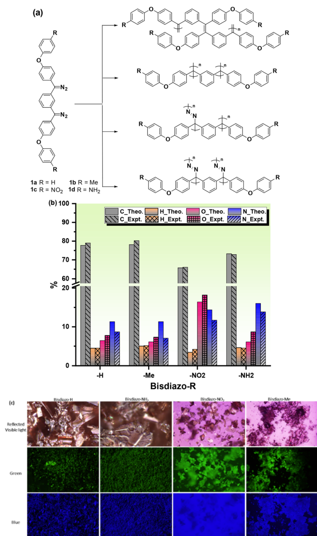
Fig. 1 (a) Chemical structures of bisdiazido-R compounds 1a–d and the possible repeating units of polymers under catalyst-free polymerization. (b) Elemental analysis and (c) optical and fluorescence images of bisdiazido-R compounds 1a–d with various terminal groups ( R = H , Me , NO_2 and NH_2 ).
