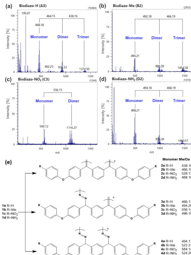
Fig. 7 FD HR-TOF MS spectra of the self-polymerized material upon heating under vacuum for (a) bisdiaz-H 1a , (b) bisdiaz-Me 1b , (c) bisdiaz-NO 2 1c and (d) bisdiaz-NH 2 1d ; (e) possible repeating unit of oligomerization structures with monoisotopic m/z .
