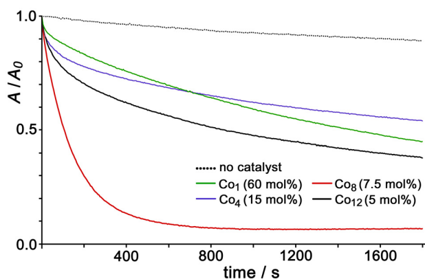
Fig. 7 Normalised UV/vis absorption data showing destruction of FLU ( 7.5 \mu\text{M} , \lambda_{\text{max}} = 489 \text{ nm} ) by oxidation with PMS (45 eq.) over time with no catalyst, \text{Co}_{12} (5 mol%), \text{Co}_8 (7.5 mol%), \text{Co}_4 (15 mol%) and \text{Co}_1 (60 mol%), with cage concentrations adjusted to give the same concentration of Co(II) centres in each case. Solvent was aqueous buffer containing TWEEN-20 surfactant (see ref. 5a) at pH 7.
