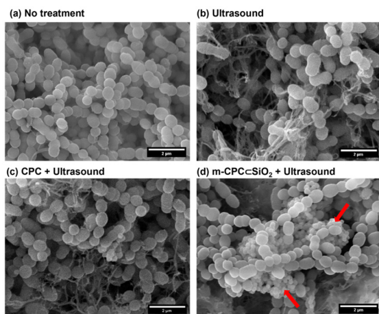
Fig. 7 SEM images of S. sanguinis biofilms showing effect of ultrasound and presence of particles. (a) no treatment; (b) treated with (ultrasound only P10 10 s); (c) CPC (14 \mu\text{g mL}^{-1} ) + ultrasound (P10, 0.27 W, 10 s) and (d) m-CPCsSiO 2 (10 mg mL -1 ) + ultrasound (P10, 10 s). Red arrows indicate the presence of m-CPCsSiO 2 . SEM magnification 10–20 kX, 20.0 kV electron beam. Scale bar represents 2 \mu\text{m} in each image.
