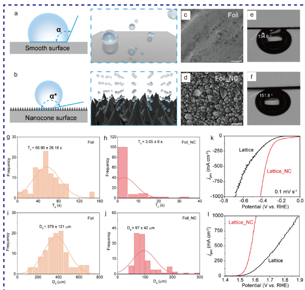
Fig. 8 Schematic illustrations show bubble contact angle, area and evolution on (a) a smooth Ni surface and (b) a NC-modified Ni surface. SEM images of (c) Foil and (d) Foil_NC. Scale bars are 1 \mu\text{m} . Digital images showing air contact angles on (e) Foil and (f) Foil_NC. Histograms illustrate the distribution of (g and h) bubble detachment time ( T_d ) and (i and j) detachment size ( D_d ) on Foil and Foil_NC substrates. LSV of Lattice and Lattice_NC electrodes collected in 1.0 M KOH at a scan rate of 0.1 \text{ mV s}^{-1} for (k) HER and (l) OER. Reproduced from ref. 81 with permission from Wiley, copyright 2023.
