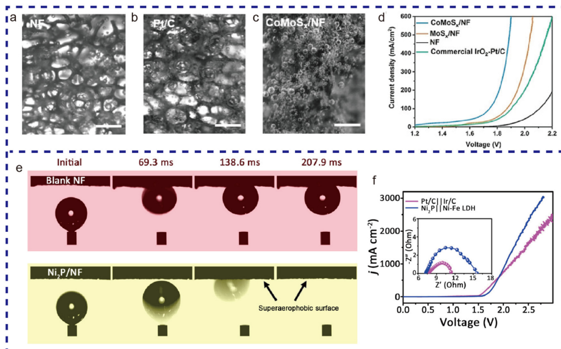
Fig. 4 Digital images showing bubbles released from (a) NF, (b) Pt/C, and (c) \text{CoMoS}_x/\text{NF} during HER at a current density of 200 \text{ mA cm}^{-2} . Scale bars are 0.5 \text{ mm} . (d) LSV for \text{CoMoS}_x/\text{NF} , \text{MoS}_x/\text{NF} , \text{IrO}_2\text{-Pt/C} , and NF electrodes at a scan rate of 5 \text{ mV s}^{-1} . Reproduced from ref. 87 with permission from Wiley, copyright 2019. (e) Digital images of hydrogen bubbles on NF and \text{Ni}_2\text{P}/\text{NF} . (f) LSV of the catalysts at a scan rate of 10 \text{ mV s}^{-1} , with the inset showing EIS Nyquist plots of the catalysts at 1.7 \text{ V} . Reproduced from ref. 101 with permission from ACS, copyright 2019.
