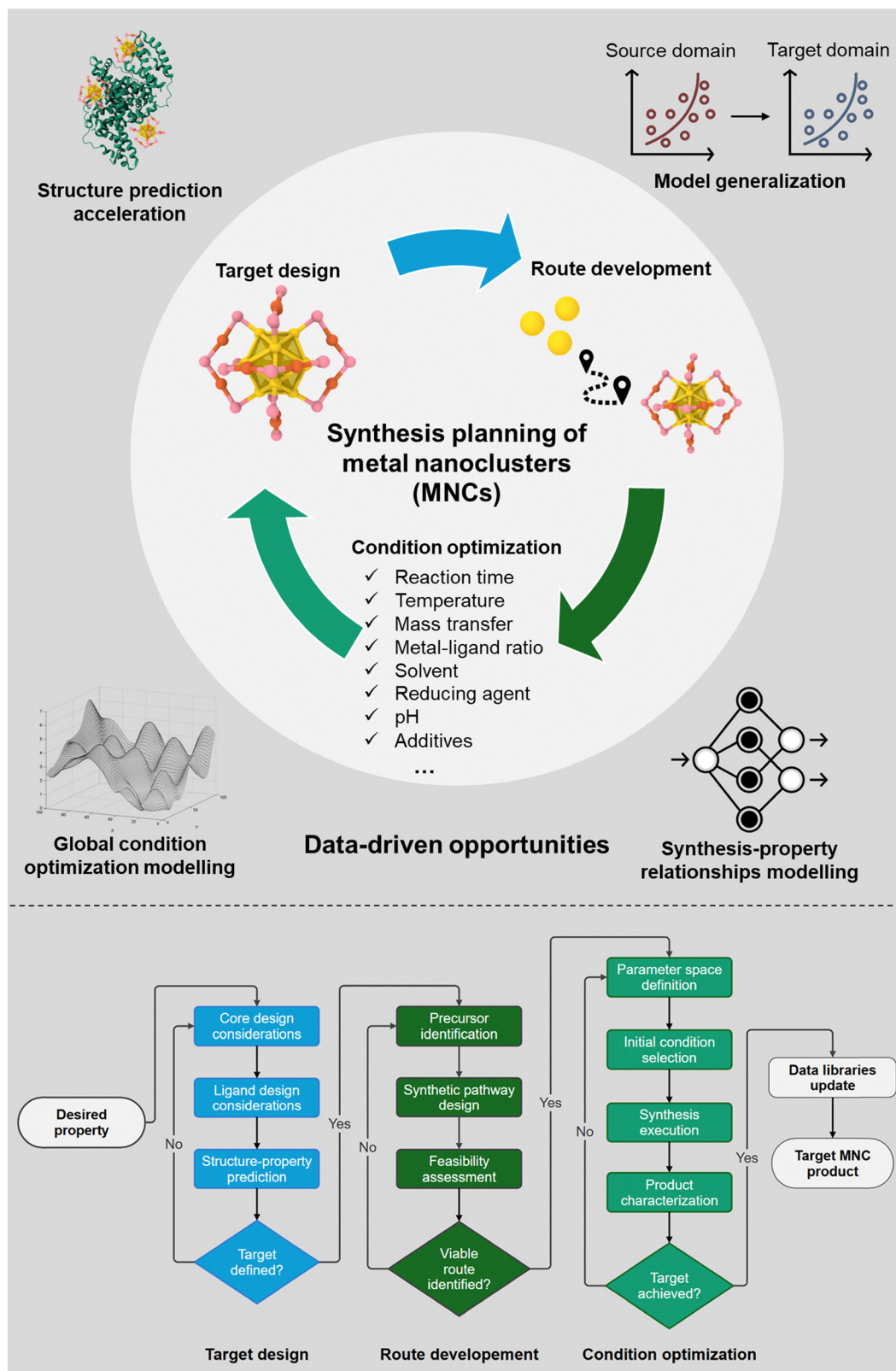
Fig. 1 Schematic overview of the synthesis planning framework of MNCs, including three main processes, namely, target design, route development and condition optimization, and the opportunities endowed by data-driven approach adoption, in terms of structure prediction acceleration, global condition optimization modelling, synthesis–property relationship modelling, and model generalization. Colour label: yellow, core Au or Au cation; orange, motif Au; pink, S. The detailed flowchart below illustrates the individual steps during the three critical stages of synthesis planning for MNCs. After each successful synthesis, all relevant data are updated to the data libraries for future MNC developments, forming an iterative cycle.
