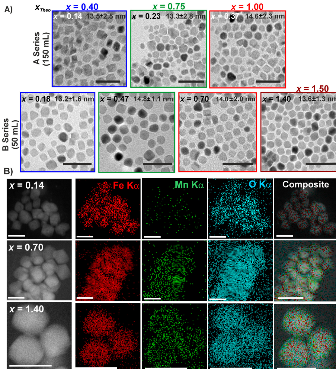
Fig. 1 (A) TEM images of \text{Mn}_x\text{Fe}_{3-x}\text{O}_4 MNPs with varying \text{Mn}^{2+} content ( x_{\text{Empirical}} = 0.14 to 1.40 ). The samples with the initial Fe/Mn precursor amount of x_{\text{Theo}} = 0.40, 0.75, 1.0 , and 1.50 are highlighted with blue, green, red, and brown boxes, respectively. Inset: Empirical x value for each sample determined by ICP-OES along with their respective size diameters. Scale bar: 50 nm. (B) STEM-EDX mapping images of \text{Mn}_x\text{Fe}_{3-x}\text{O}_4 MNPs with the lowest, medium, and highest content of \text{Mn}^{2+} ( x_{\text{Empirical}} = 0.14, 0.70, 1.40 ). Scale bar: 50 nm ( x_{\text{Empirical}} = 0.14 and 0.70 ), 20 nm ( x_{\text{Empirical}} = 1.40 ).
