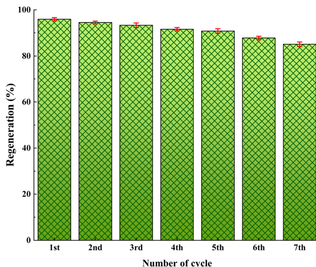
Fig. 1 Recyclability performance of \text{UiO-66-NH}_2\text{@SA-PS/CuI} .
