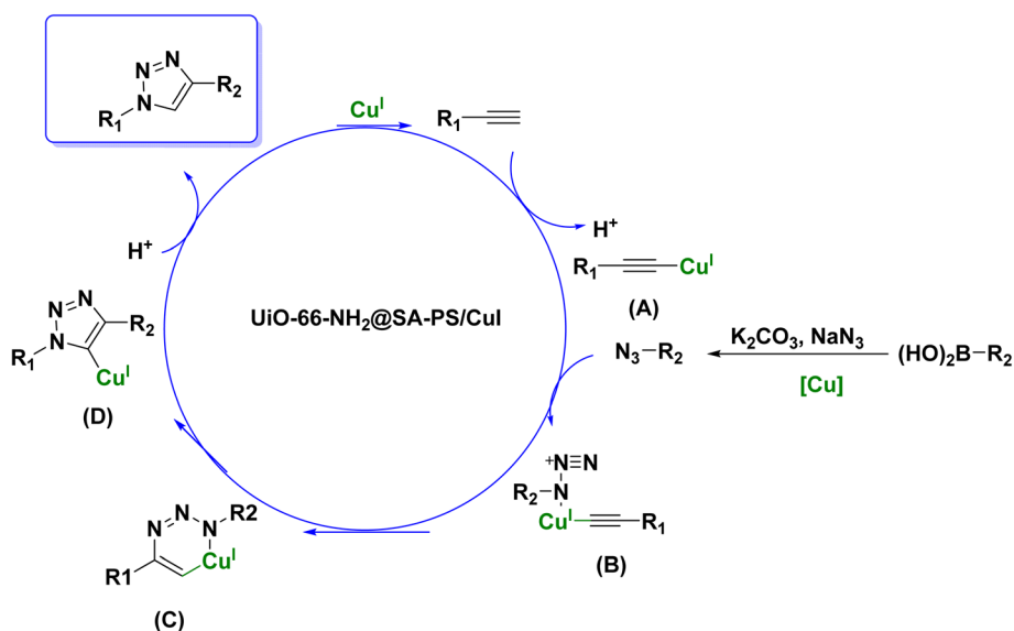
Scheme 4 Proposed mechanism for the \text{UiO-66-NH}_2\text{@SA-PS/CuI} -catalyzed CuAAC reaction.
