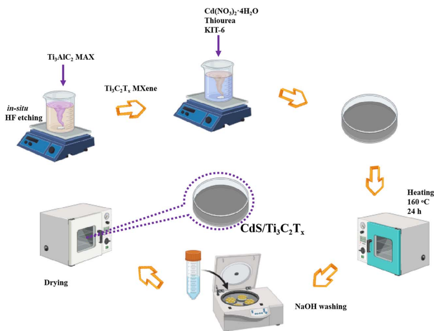
Fig. 1 Synthesis of CdS/Ti_3C_2T_x composites (schematic).
