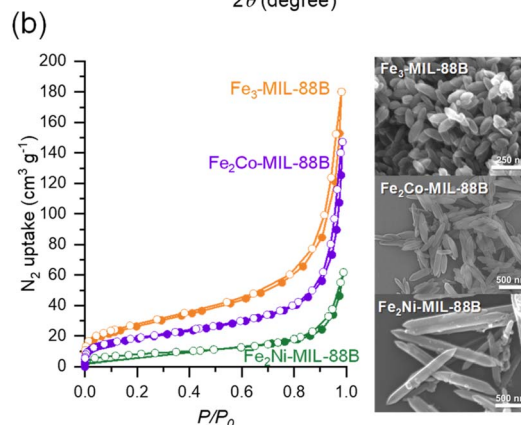
Fig. 2 (a) PXRD patterns of \text{Fe}_3 -MIL-88B, \text{Fe}_2\text{Co} -MIL-88B, and \text{Fe}_2\text{Ni} -MIL-88B collected after isolation from DMF. (b) \text{N}_2 isotherms at 77\text{ K} and SEM images of \text{Fe}_3 -MIL-88B, \text{Fe}_2\text{Co} -MIL-88B, and \text{Fe}_2\text{Ni} -MIL-88B.
