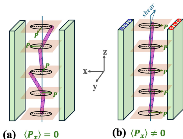
Fig. 6 Illustration of the shear deformation of the director structure and the induction of net polarization in the SmC* phase. The smectic layers are parallel to the x-y plane. The tilt plane rotates from one layer to the other. (a) Undisturbed helical structure where the macroscopic polarization is averaged out. (b) Due to the action of the shear along y, the axial symmetry of the configuration is broken, and a non-zero polarization component appears along x. Arrows indicate the spontaneous polarization \vec{P} , which is normal to the tilt plane (the plane determined by the layer normal and the projection of the tilt direction, the so-called c-director).
