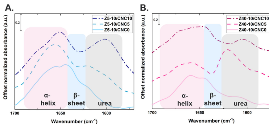
Fig. 5 PTIR investigation of the amide I region ( 1700\text{--}1600\text{ cm}^{-1} ) of A. Z5-10/CNC series and B. Z40-10/CNC series as a function of CNC weight fraction.
