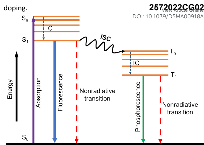
Figure 2. Schematic diagram of fluorescence and phosphorescence emission mechanism. Abbreviations: IC, internal conversion; ISC, intersystem conversion.
