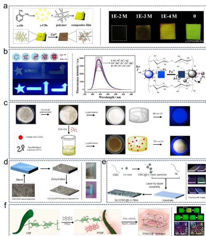
Figure 4. Design strategy and phenomena for achieving extrinsic fluorescence of cellulose. (a) Preparation process of \gamma -CD/PVA/CMC film and fluorescent image of the film interacting with \text{Cu}^{2+} . [Reproduced with permission from ref. 24 Copyright 2013 The Royal Society of Chemistry.] (b) Fluorescence imaging of bacterial cellulose loaded carbon dots composite materials and the mechanism of specific recognition of \text{Fe}^{3+} . [Reproduced with permission from ref. 25 Copyright 2017 Elsevier Ltd.] (c) Fabricating process and fluorescent properties of nanofibrillated cellulose and NFC loaded CDs composite. [Reproduced with permission from ref. 26 Copyright 2020 Elsevier B.V.] (d) Preparation process of CNC/ZnS/PVA nanocomposite film and the fluorescent spectra. [Reproduced with permission from ref. 27 Copyright 2019 Springer Nature B.V.] (e) Preparation process of Qc/(CMC@In) films and fluorescence imaging. [Reproduced with permission from ref. 28 Copyright 2017 Elsevier Ltd.] (f) Production process of PVA/CNF hydrogel and the fluorescent image of anti-counterfeiting. [Reproduced with permission from ref. 29 Copyright 2024 Elsevier B.V.]
