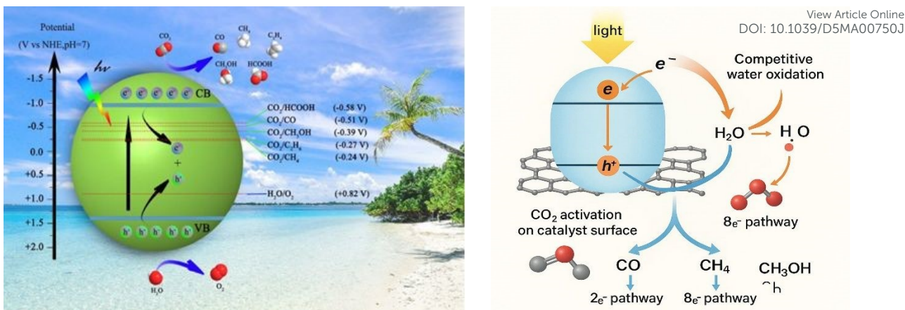
Fig. 2 (A) Band edge alignment and redox potentials for photocatalytic \text{CO}_2 reduction with \text{H}_2\text{O} , (B) General mechanism of graphene-based photocatalytic \text{CO}_2 reduction pathways, Reprinted with the Ref. [22], Copyright@2020, RSC.
