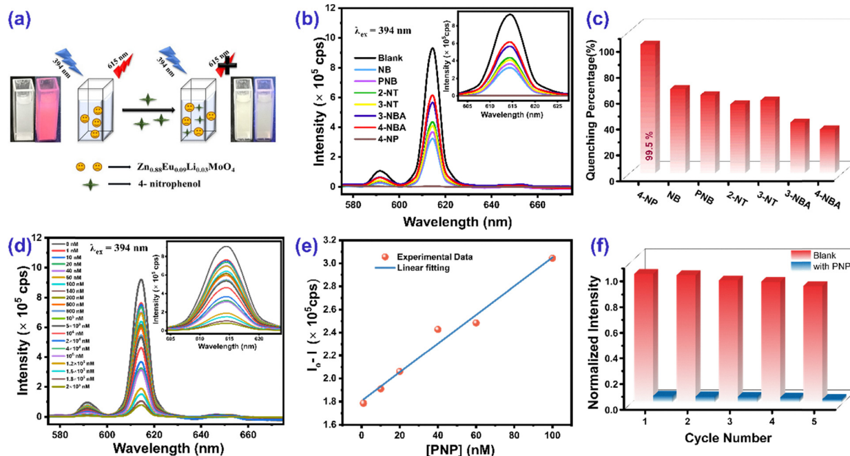
Fig. 8 (a) Schematic illustration for 4-nitrophenol sensing using the Zn 0.88 Eu 0.09 Li 0.03 MoO 4 (ZELMO) phosphor. (b) The luminescence intensity of ZELMO dispersed in aqueous solutions of different nitroaromatic compounds excited with 394 nm. (c) Bar diagram to show the nitro aromatic compound selectivity of ZELMO in deionized water. (d) The luminescence response of ZELMO to different concentrations of 4-NP (0–200 \mu M) in deionized water. (e) Plot of I_0 - I versus increasing concentrations of 4-NP to calculate the limit of detection. (f) Original (red) and quenched (blue) luminescence intensity of ZELMO at 615 nm recycled after sensing experiments for 4-NP.
