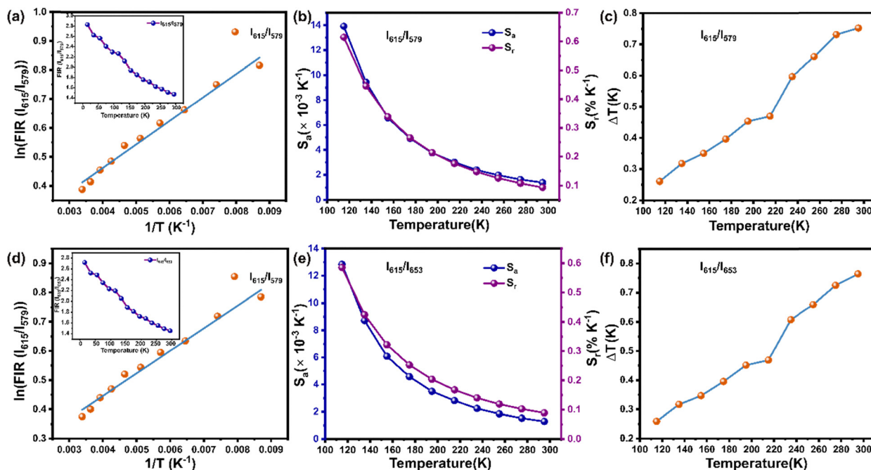
Fig. 11 In(FIR) vs. 1/T plot for (a) I_{615}/I_{579} , and (d) I_{615}/I_{653} (the inset shows the respective FIR vs. T plots). Temperature dependence of absolute sensitivity ( S_a ) and relative sensitivity ( S_r ) for (b) I_{615}/I_{579} , and (e) I_{615}/I_{653} . Variations in temperature uncertainty ( \Delta T ) with temperature for (c) I_{615}/I_{579} , and (f) I_{615}/I_{653} .
