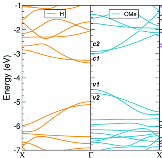
Fig. 8 DFT band structures of GNR-OMe ( 8.3 ) (R = OMe; blue, right) and GNR-H (R = H; orange, left). The two band structures are aligned to the vacuum level, which is set to zero. 69 Reproduced from ref. 69 with permission from [RSC], copyright [2022].
