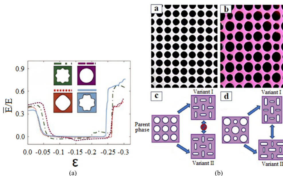
Fig. 2 Pattern changes with variable stiffness. (a) Hole shapes. (b) Array of holes: (a) holey sheets. (b) Biholar sheets. (c) Phase transitions for holey sheets. (d) Phase transitions for biholar sheets. 37 This figure was reprinted with permission from Wang et al. 37 Copyright 2023 Frontiers Media SA.
