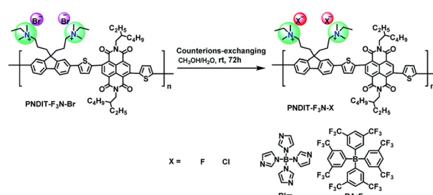
Fig. 21 Chemical structure of PNDDIT-F 3 N-X.
