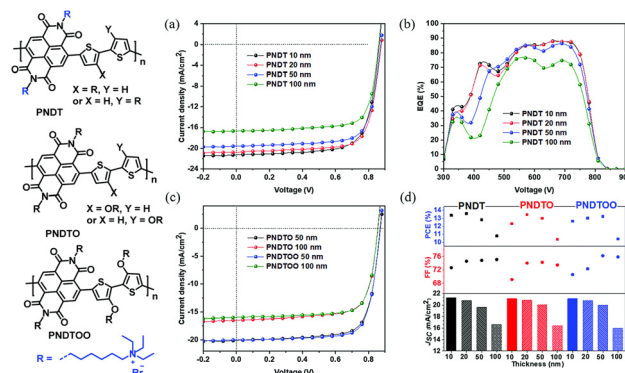
Fig. 20 J - V characteristics (a) and (b) the EQE curves of PBDB-2Cl:ITIC-2F-based photovoltaic devices with PNDDT as the ETM; (c) J - V characteristics of PBDB-2Cl:ITIC-2F-based photovoltaic devices with PNDDTO and PNDDTOO as ETMs; and (d) the summary of photovoltaic parameters for PBDB-2Cl:ITIC-2F-based photovoltaic devices with these CPEs as ETMs. 122
