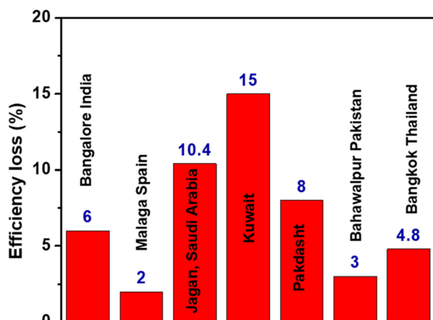
Fig. 2 Effect of dust on solar panel efficiency. 19
