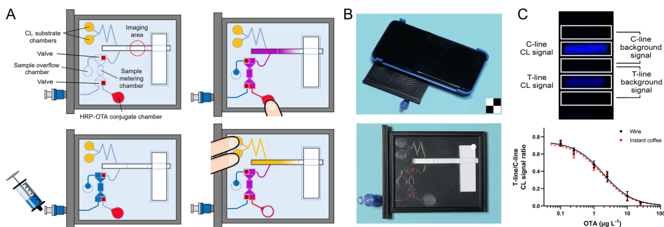
Fig. 46 LFIA-ready membrane in a cartridge with finger-actuated reagent pouches for the CL-based detection of ochratoxin A (OTA) in wine and coffee samples. (A) Schematic overview of LFIA analysis. Sample is loaded, transferred, and mixed with various reagents on-chip before being injected onto the LFIA strip. (B) Photographs of the physical device and chip. (C) Example of a smartphone-acquired CL image of the LFIA and a calibration plot for OTA obtained in wine and instant coffee. Adapted with permission from ref. 528 Copyright 2021 Elsevier B.V.
